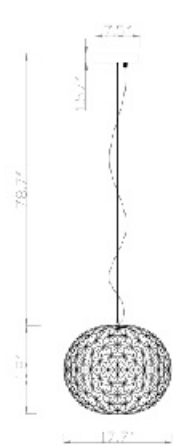
OC16P18S 32W LED 3000K DIMMABLE
